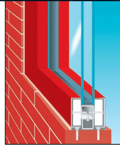
SuperLite II-XL 120 minute in SAFTI fire GPX Framing
